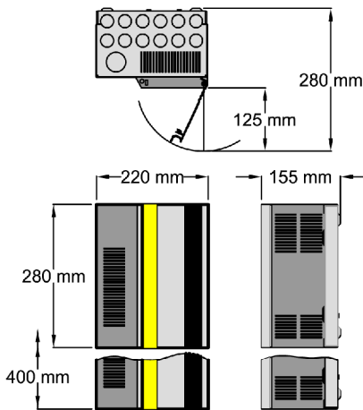
SCI0405 D version - 400x220x155mm RCBO & RCBOX version - 340x255x155mm
